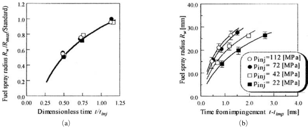
Fig. 4 Temporal change in spray radius R_w , Parameter : Injection pressure p_{inj} ( Q_{inj}=12.0 [mg], T_w=550 [K], \rho_a=12.3 [kg/m 3 ], Z_w=40 [mm])
