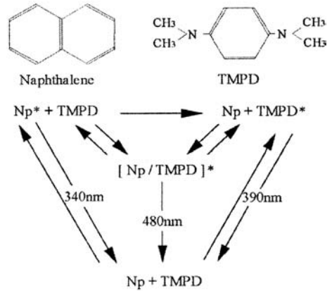
Fig. 2 Schematic summary of naphthalene and TMPD exciplex system
