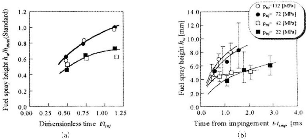
Fig. 5 Temporal change in spray height h_w , Parameter : Injection pressure p_{inj} ( Q_{inj}=12.0 [mg], T_w=550 [K], \rho_a=12.3 [kg/m 3 ], Z_w=40 [mm])
